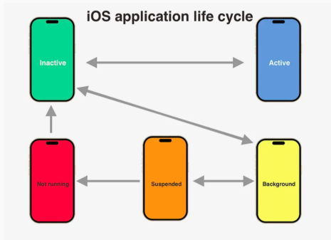
Figure 13: App lifecycle
