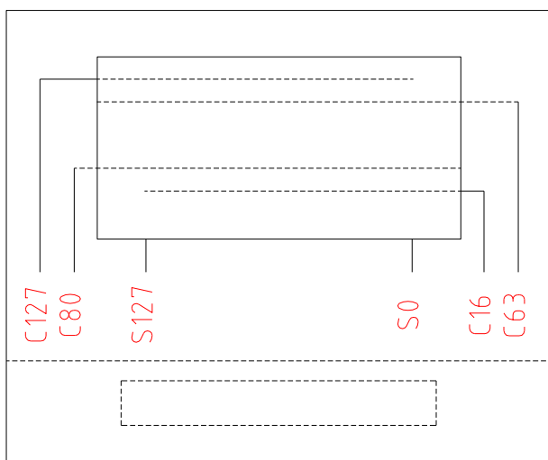
COM&SEG LAYOUT
