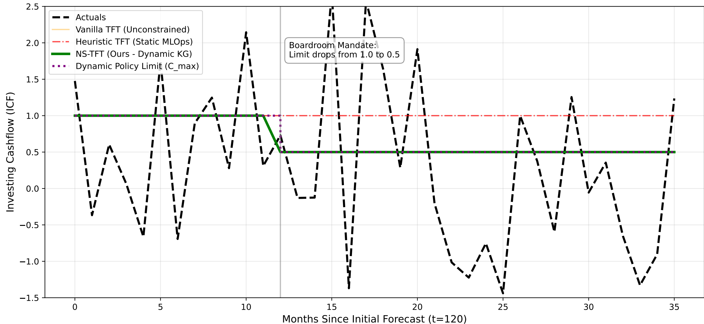
Experiment 3: Dynamic Knowledge Extraction Under Structural Shock
