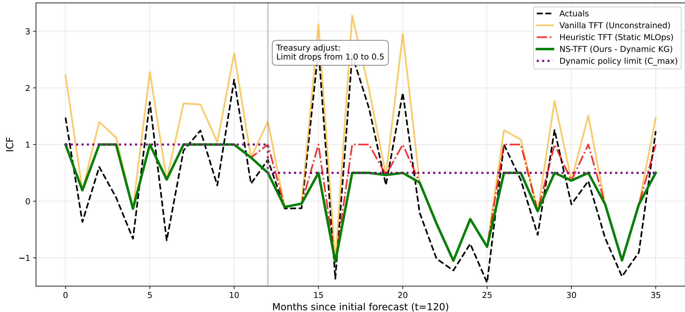
Experiment 3: Dynamic Knowledge Extraction & Shocks (ICF)
