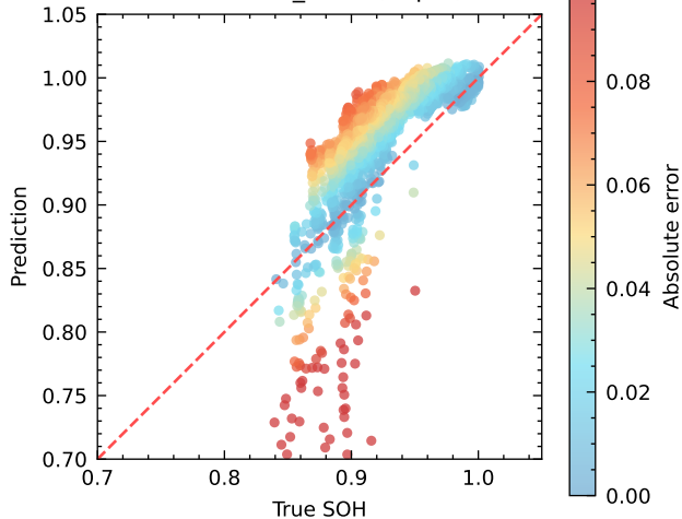
Arrhenius_T45C (Exp 1)
