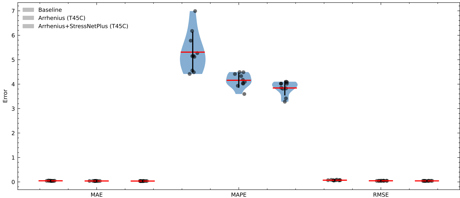
CALCE (10 runs): Baseline vs Arrhenius(T) vs Arrhenius+StressNetPlus
