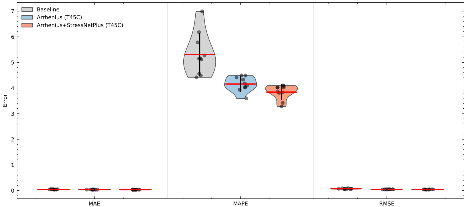
CALCE (10 runs): Baseline vs Arrhenius(T) vs Arrhenius+StressNetPlus
