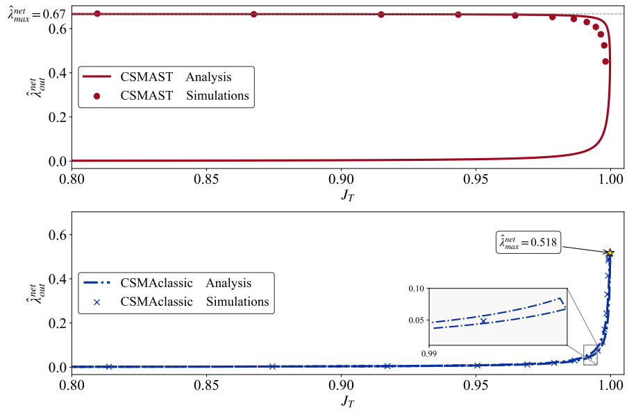
图 4-7 CSMAST 与经典 CSMA 的吞吐量-公平性轨迹对比 ( n = 100, \tau_S = 5, \tau_F = 3, \tau_I = 1, T = 10^6 )
