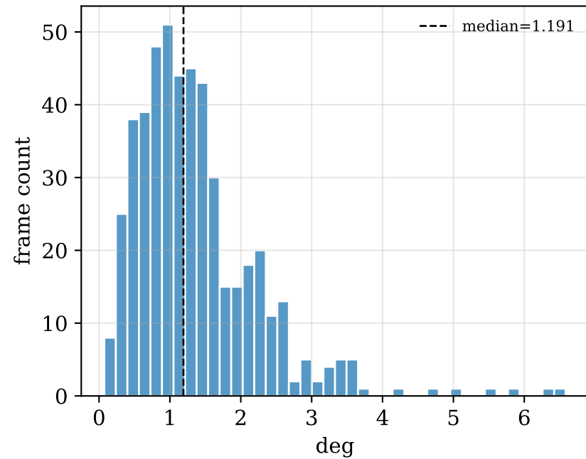
Rotation error (geodesic)
