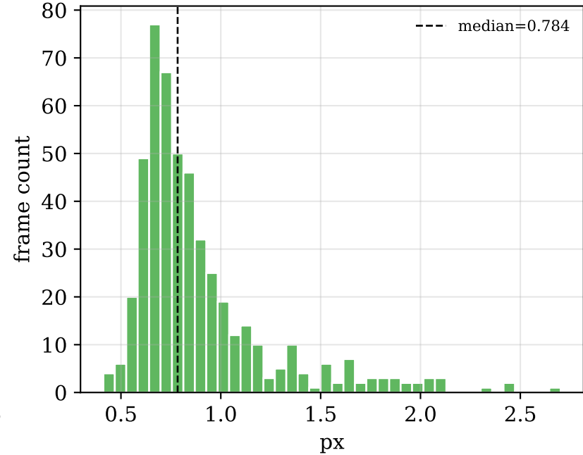
Mean reprojection error
