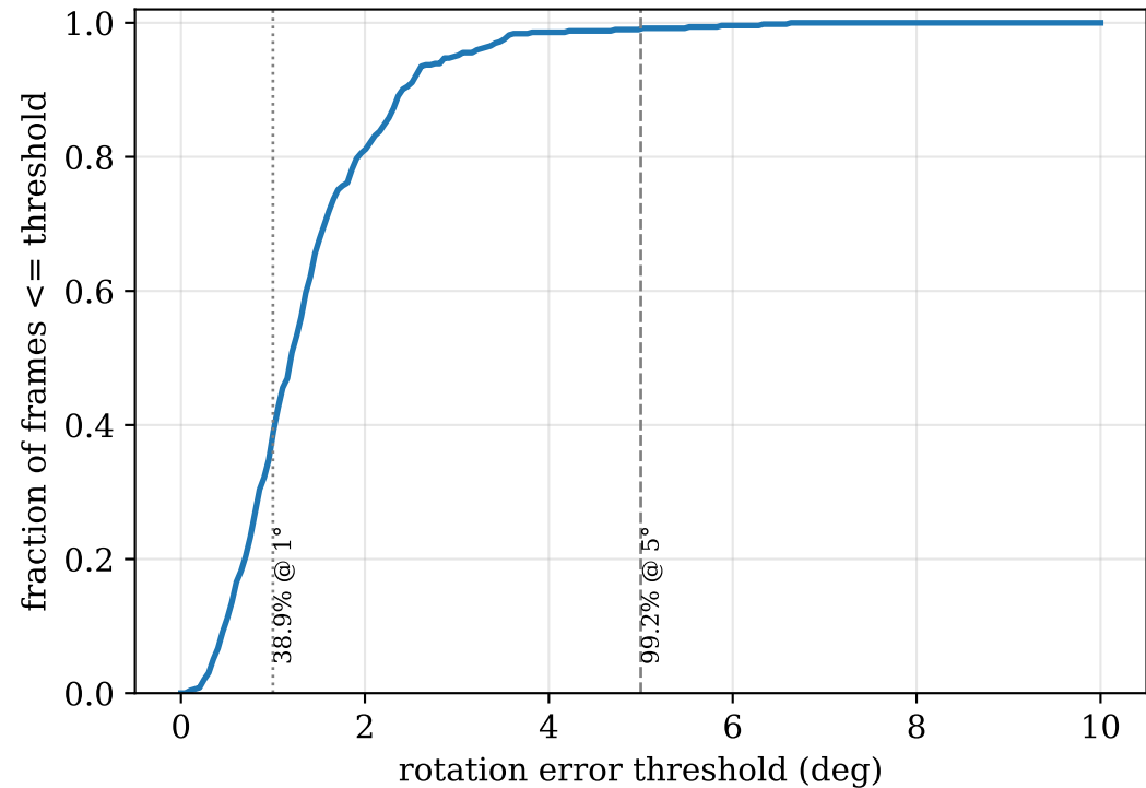
Rotation accuracy-at-threshold
