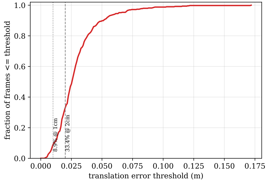
Translation accuracy-at-threshold
