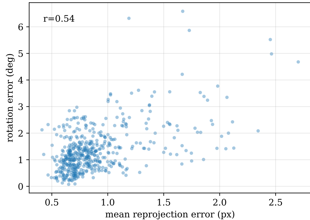
Rotation error vs reprojection error
