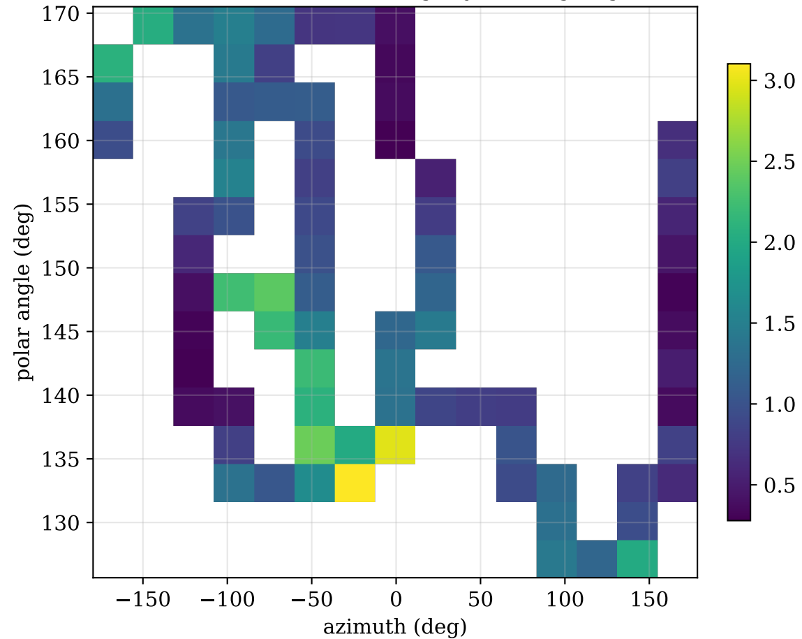
Mean rotation error (deg) by viewing angle
