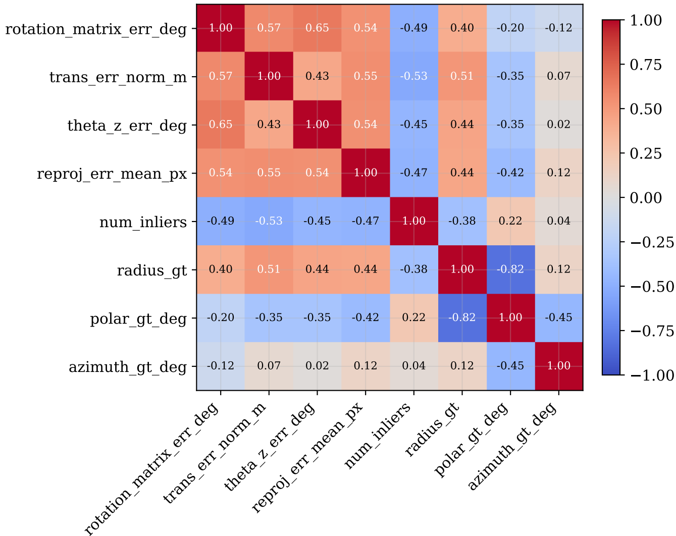
Correlation matrix: errors vs PnP/viewing diagnostics
