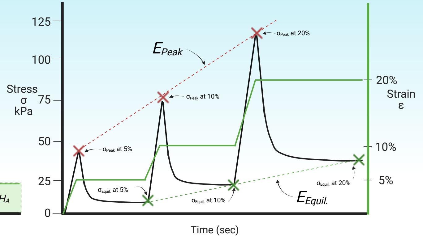
Stress Relaxation Curve
