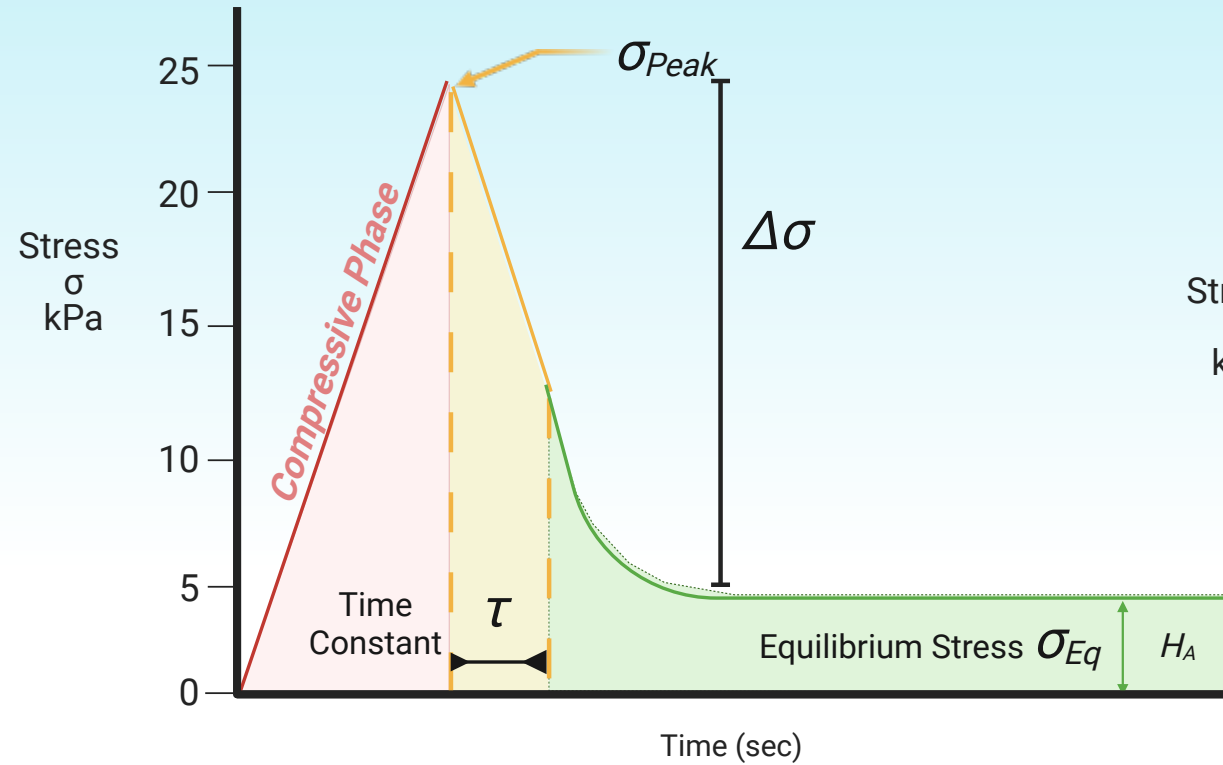
Stress Relaxation Metrics
