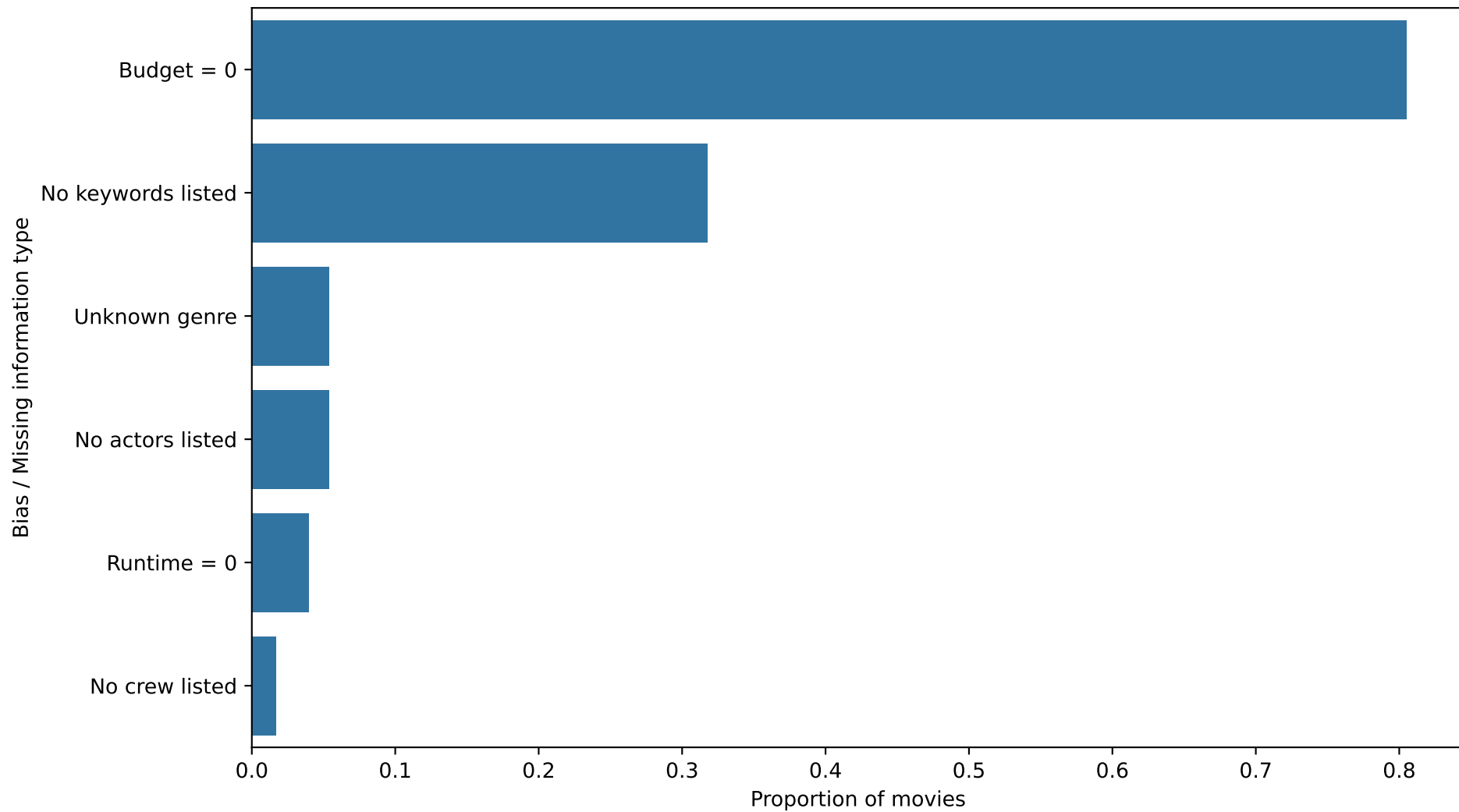
Biases and Missing Information in Dataset
