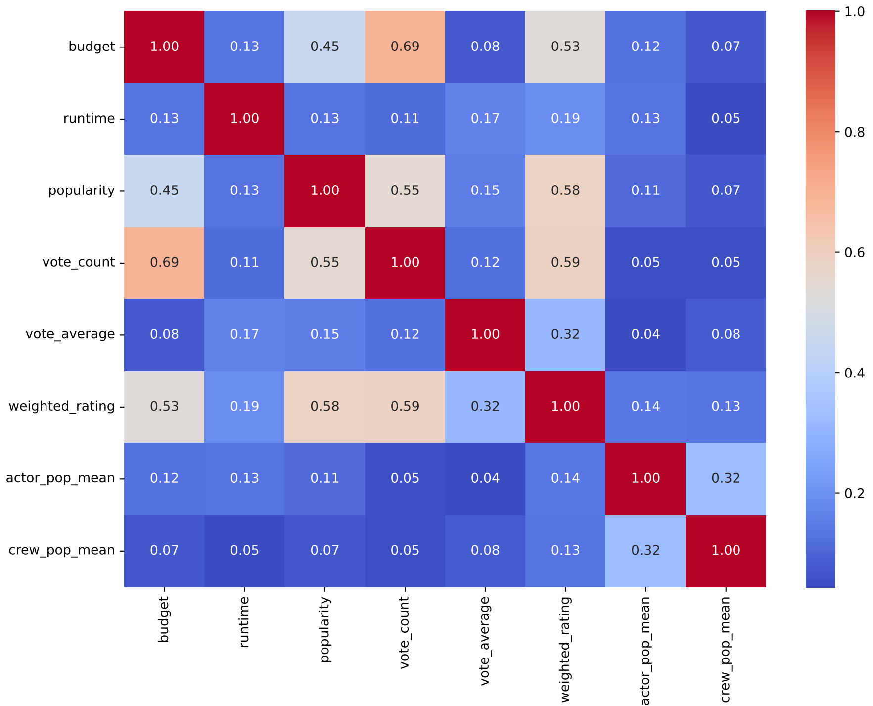
Correlation Between Numeric Features
