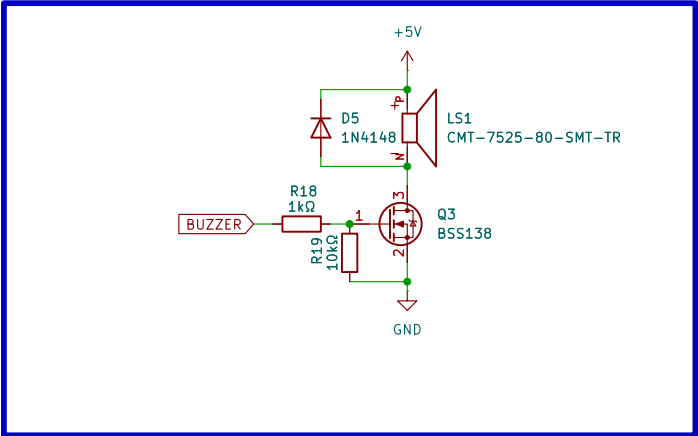
BUZZER
