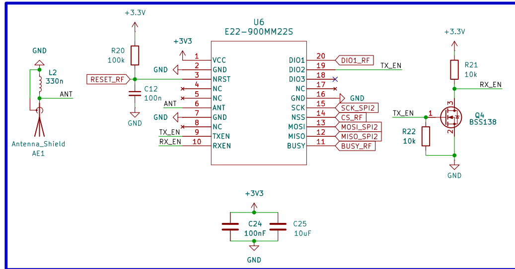
RF
