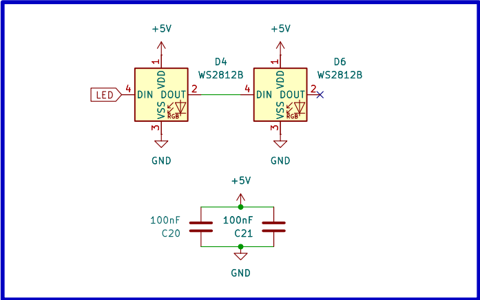
LED ADRESSABLE
