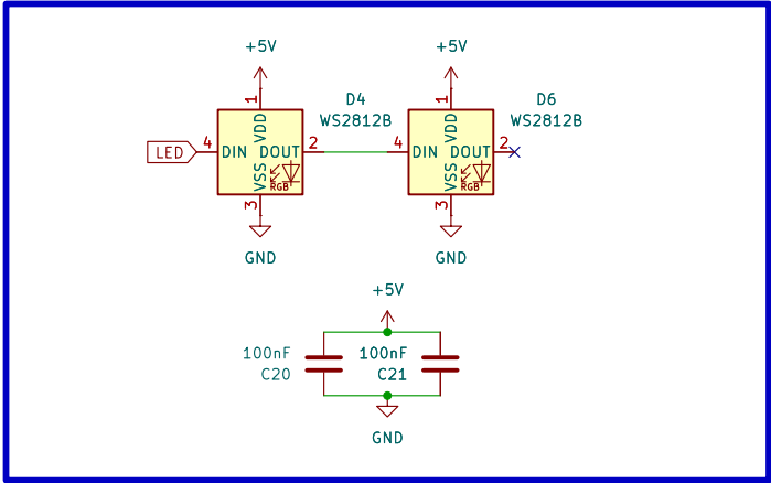
LED ADRESSABLE
