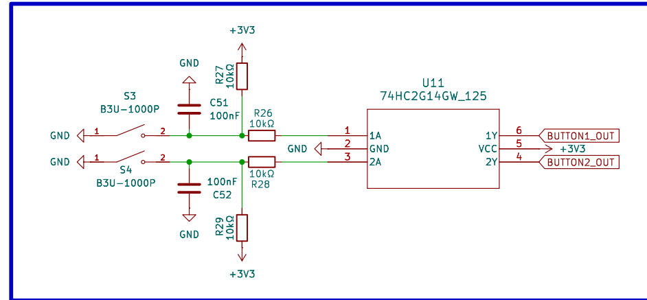
BUTTON ON SCHMITT TRIGGER
