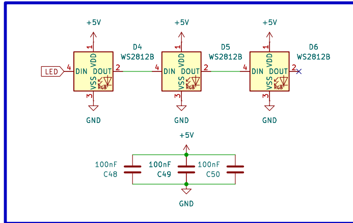
LED ADRESSABLE
