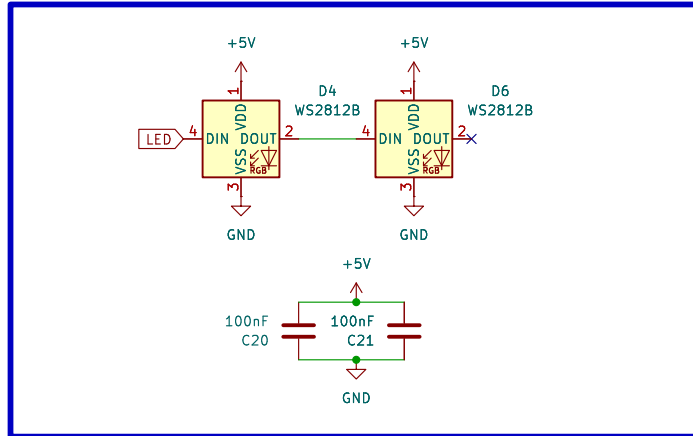
LED ADDRESSABLE
