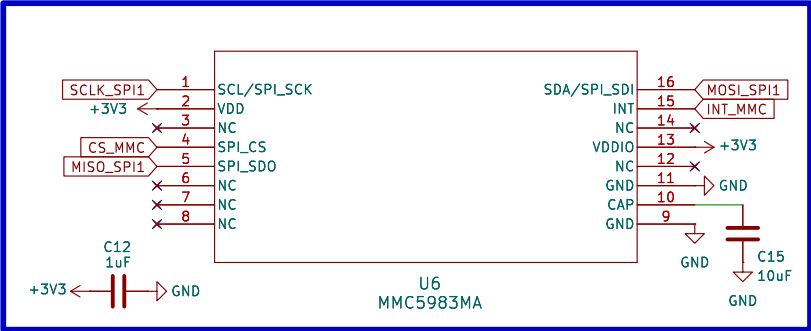
MAGNETOMETER
