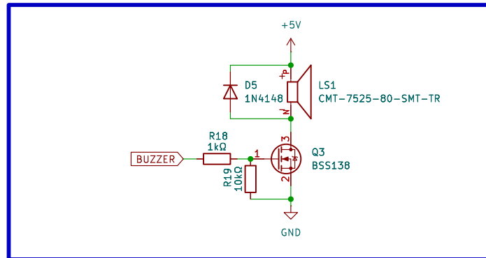
BUZZER
