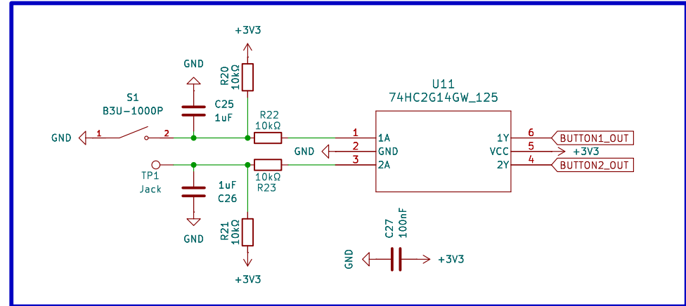
BUTTON ON SCHMITT TRIGGER
