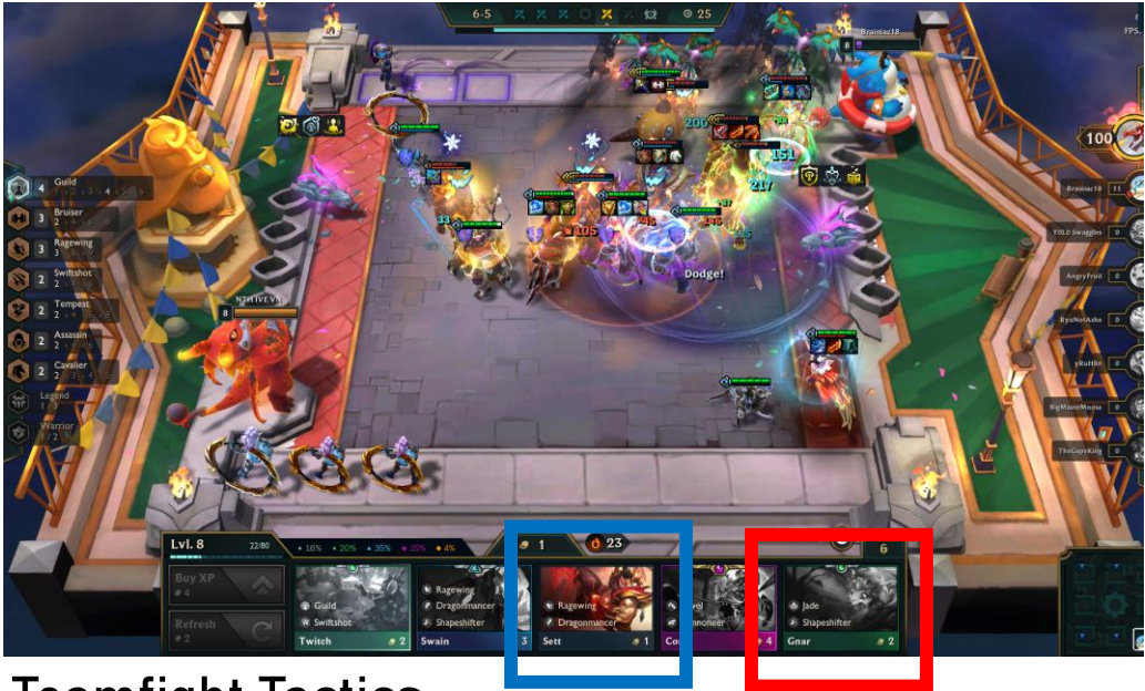
Teamfight Tactics
