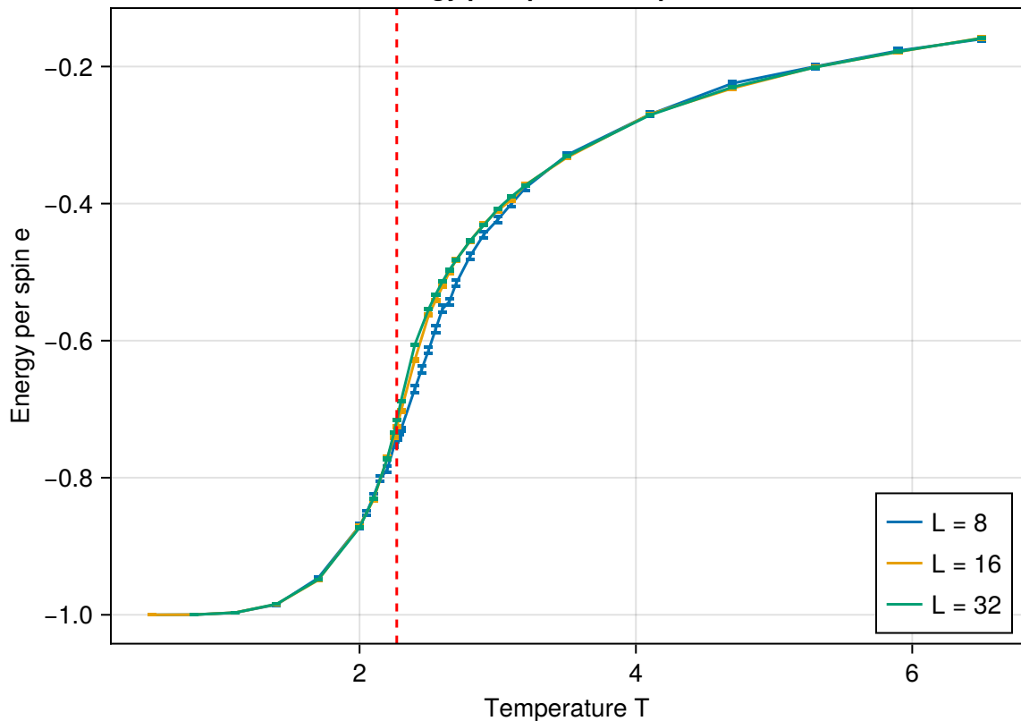
Energy per spin vs Temperature
