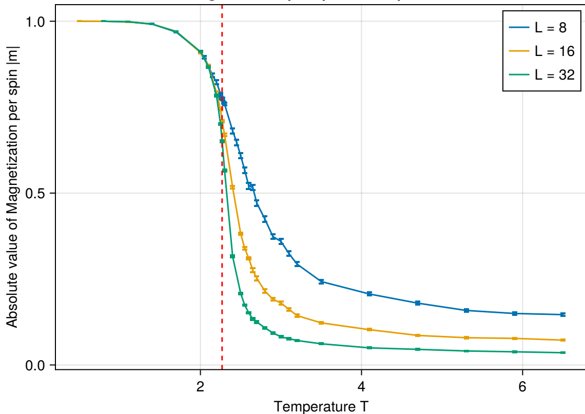
Magnetization per spin vs Temperature
