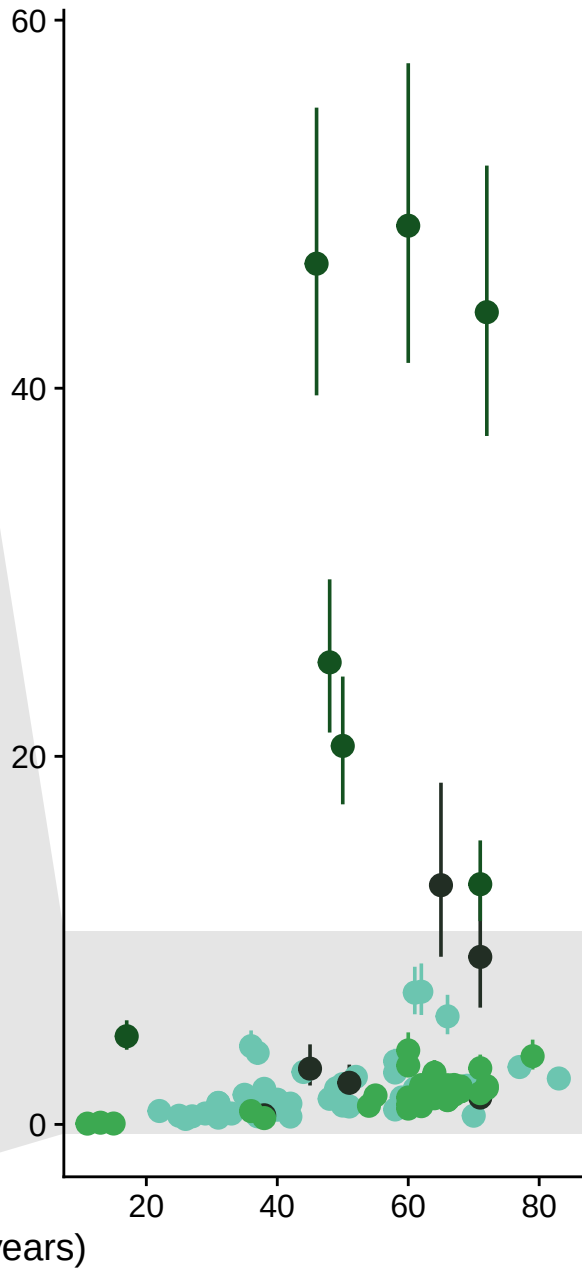
number of cells with double APC driver mutations – fraction method
