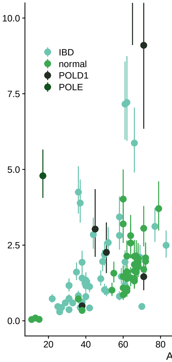
number of cells with double APC driver mutations – fraction method
