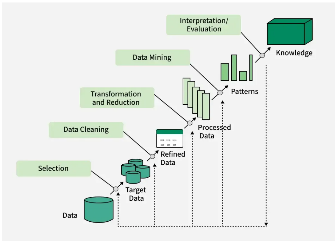
FIGURE 3.1 – Processus Knowledge Discovery in Databases (KDD).
