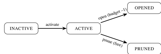
Figure 3: The controller’s state machine (§3.4). Opening a node consumes budget and may activate inactive neighbors ( reading_order , or across a document boundary via links_to/continues ); pruning is free, applied to any node still ACTIVE once budget is exhausted.
