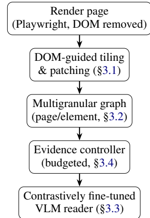
Figure 2: Pipeline overview. Rendering and tiling happen once per page; the evidence controller runs once per query, deciding which graph nodes the reader opens.
