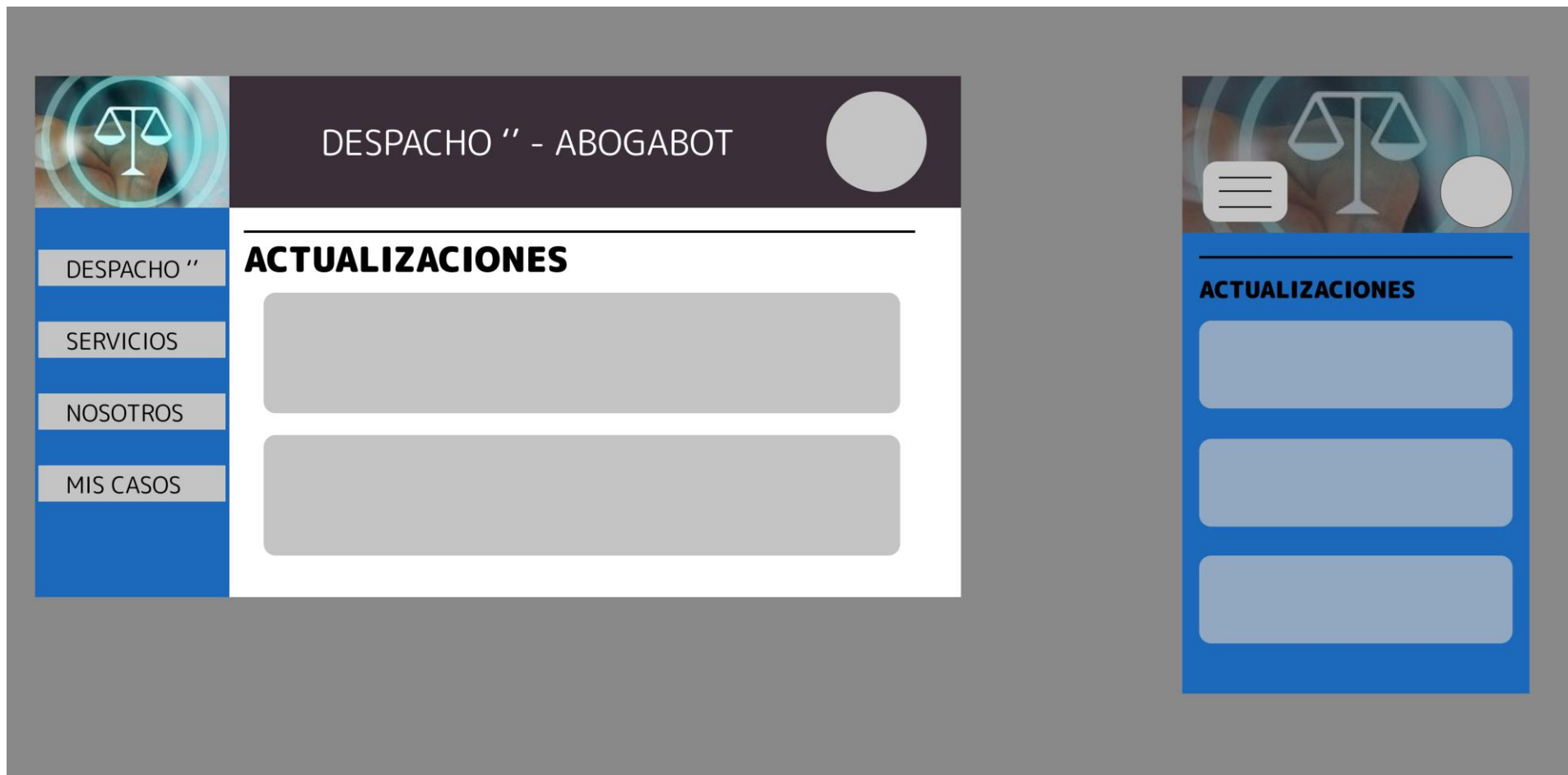
FIGURA 3: USER DASHBOARD
