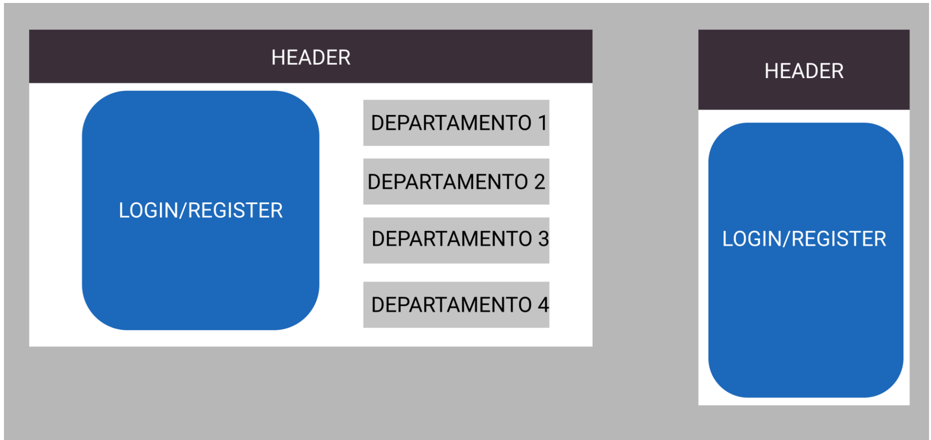
FIGURA4: ADMIN LOGIN
