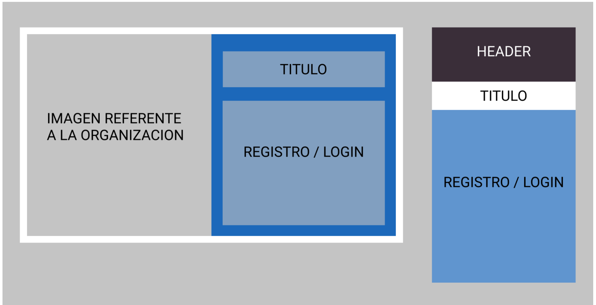
Figure1: USER LOGIN
