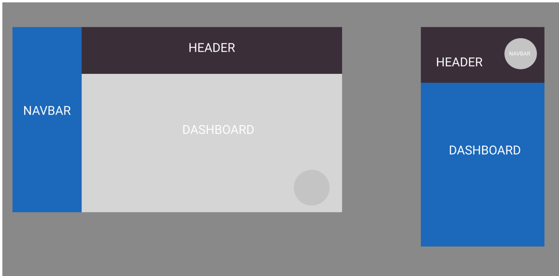
FIGURA 2: USER DASHBOARD
