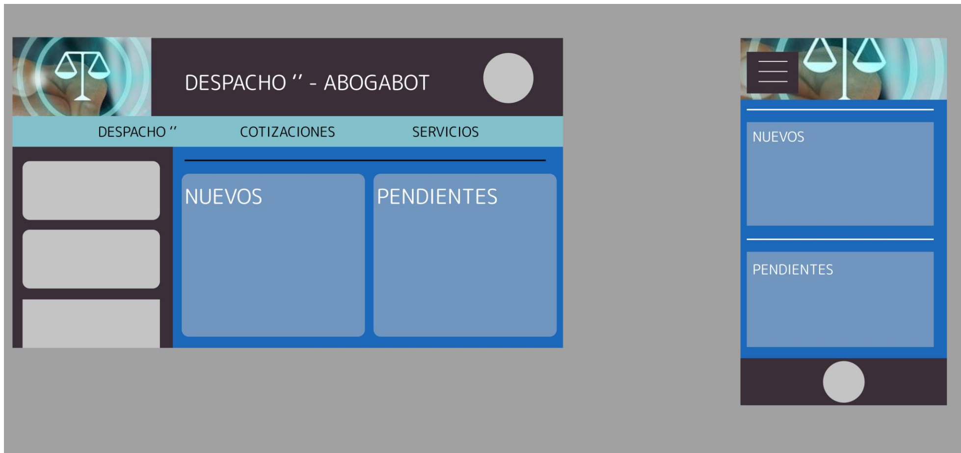
FIGURA 5: ADMIN DASHBOARD
