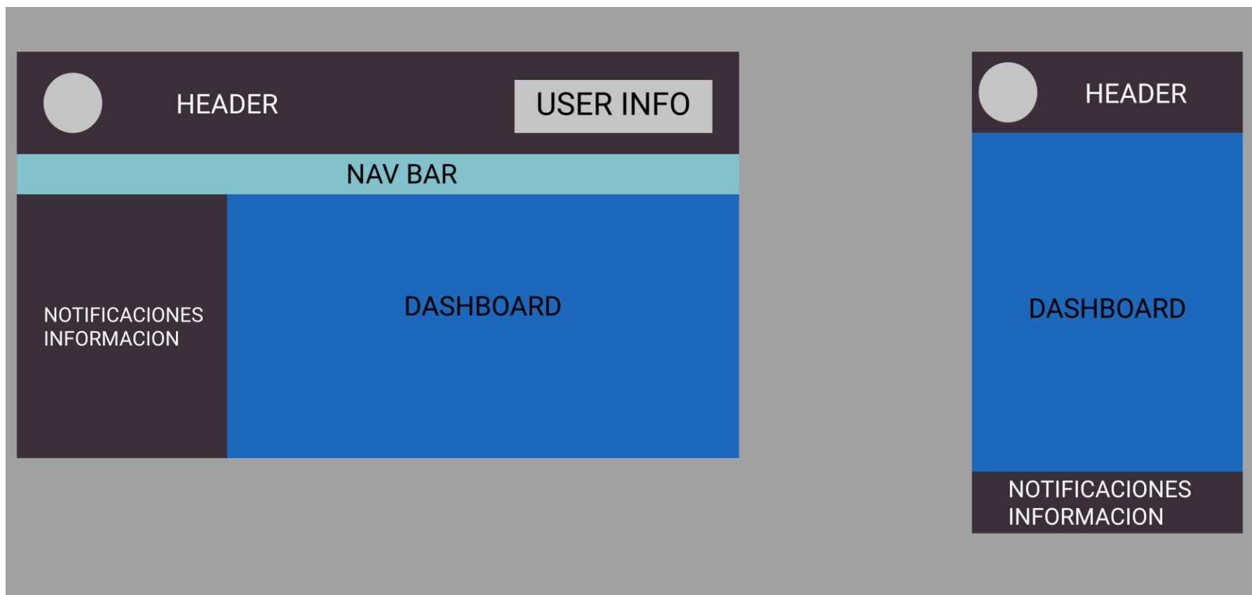
FIGURA5: ADMIN DASHBOARD
