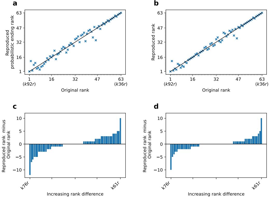
Figure 3: Probabilistic ending tournament. Comparison between the original tournament rankings and reproduced rankings under probabilistic and fixed match lengths. Panels a and b show the reproduced ranks against the original ranks for the probabilistic-ending and fixed-length implementations, respectively. Panels c and d show the corresponding rank differences relative to the original tournament. Despite small variations for some strategies, the overall tournament structure and the identities of the highest- and lowest-ranked strategies remain unchanged. Panels b and d are also shown in the main text (Figure 1); however, we reproduce them here to allow for direct comparison with the probabilistic-ending tournament results.
