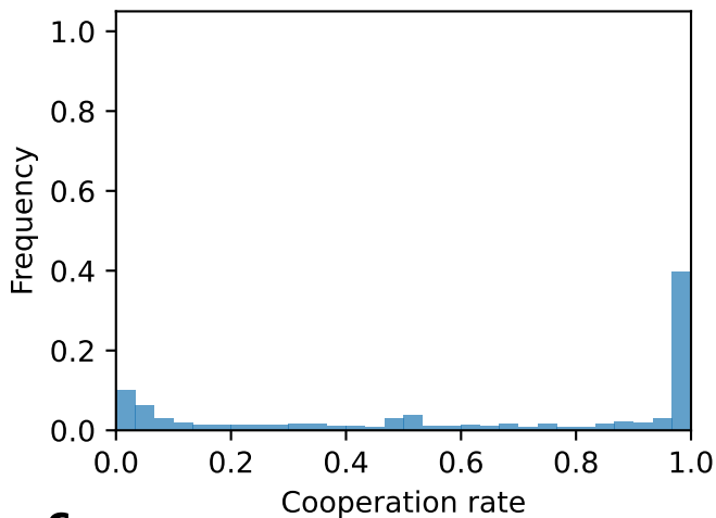
a Axelrod-Python Tournament
