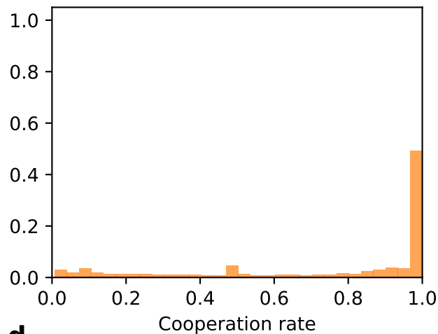
b Axelrod's Original Tournament
