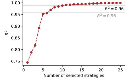
Supplementary Figure 2: Reproduction of Axelrod’s linear model. a , The representative strategies and their effect on average score. We reproduce the linear model described in [1], which reports R^2 = 0.979 . Fitting a new model to the same five strategies yields R^2 = 0.957 . The fit is an ordinary least squares linear regression; the reported R^2 values are coefficients of determination, and no significance tests or multiple-comparison adjustments were applied. b , R^2 as a function of the number of strategies included (subset size), obtained using recursive feature elimination (RFE) [3]. Starting from the full set of strategies, we iteratively remove the least informative one, refit the model, and record the resulting R^2 . For each subset size (from 1 to 25), the subset yielding the highest R^2 is retained. The estimated R^2 rises rapidly from about 0.75 to 0.95 as the number of included strategies increases from 1 to 5, after which improvements are smaller.
