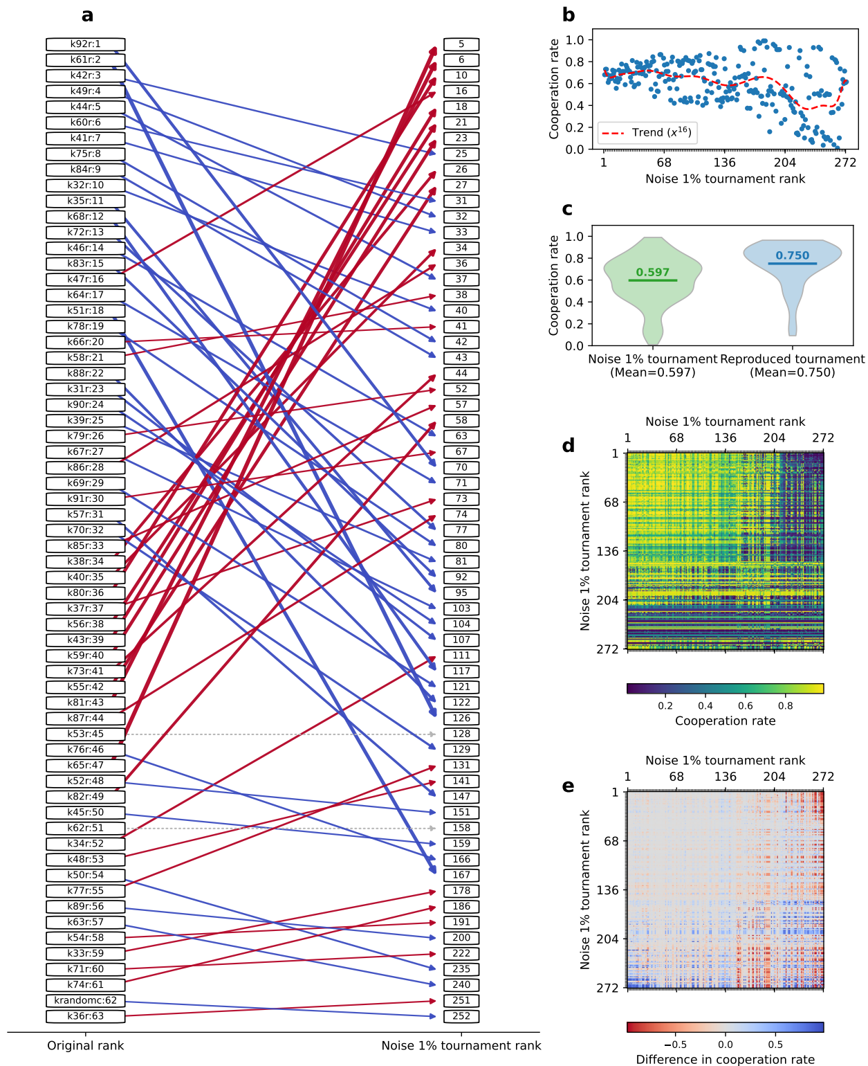
Figure 9: Reproduction of Axelrod's second tournament with the addition of the strategies from the Axelrod-Python and with noise 1%. Similar to Figure 6,
