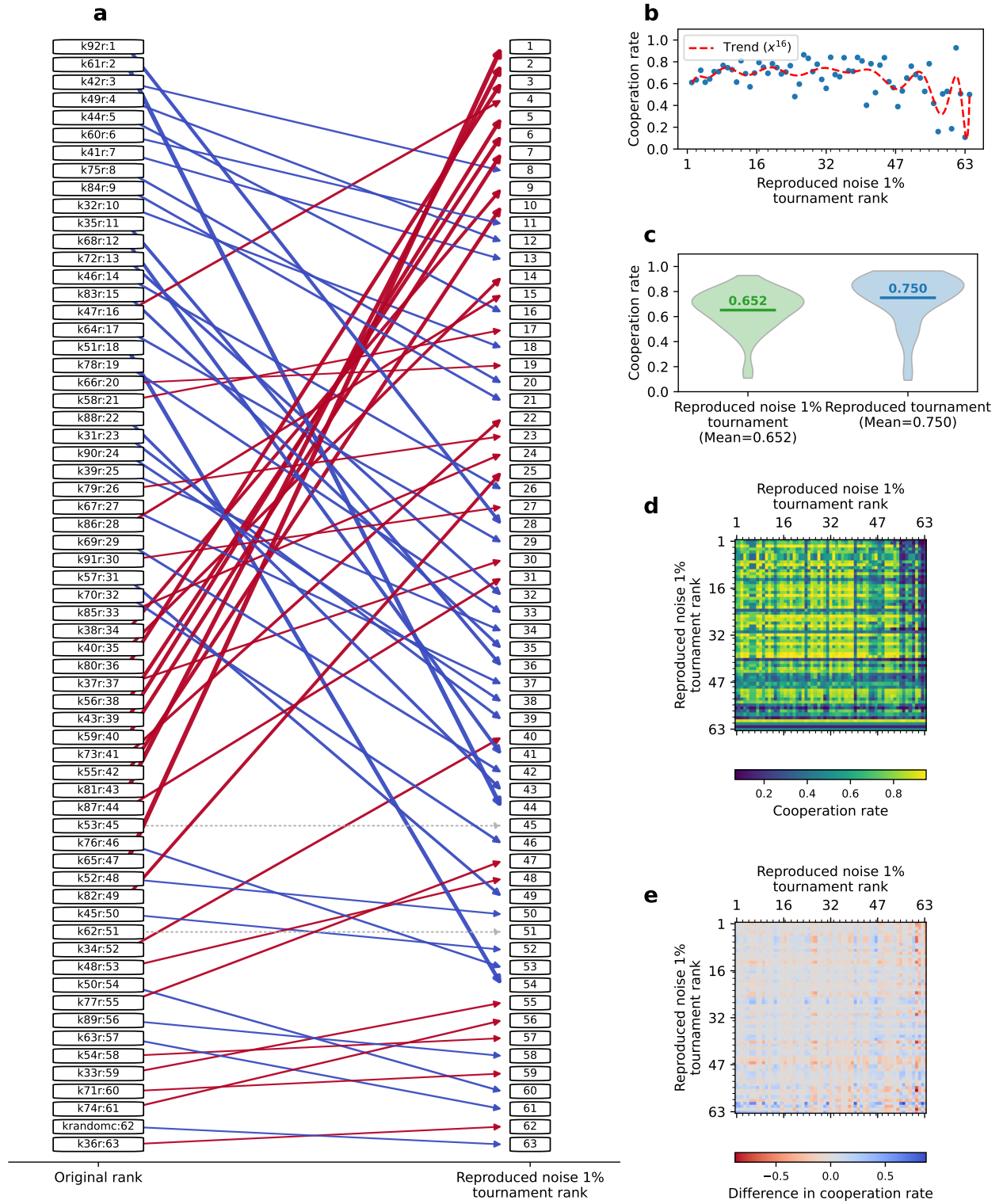
Figure 6: Axelrod's second tournament with 1% noise. a , Comparison of the original rankings with those obtained in our replication under noise. In the left column, strategies are ordered by their reproduced ranks, and arrows indicate their ranks in the noisy tournament (right column). b , Cooperation rates of strategies ordered by rank in the reproduced tournament with noise. The top-performing strategies show cooperation rates ranging from 0.6 to 0.8. c , Tournament ranks across all repetitions with noise compared to the reproduced tournament without noise. We also plot the average cooperation rate. d , Pairwise cooperation rates between strategies in the reproduced tournament without noise and with 1% noise. e , Differences in cooperation rates for each pair of strategies, again ordered by their rank in the reproduced tournament with noise.
