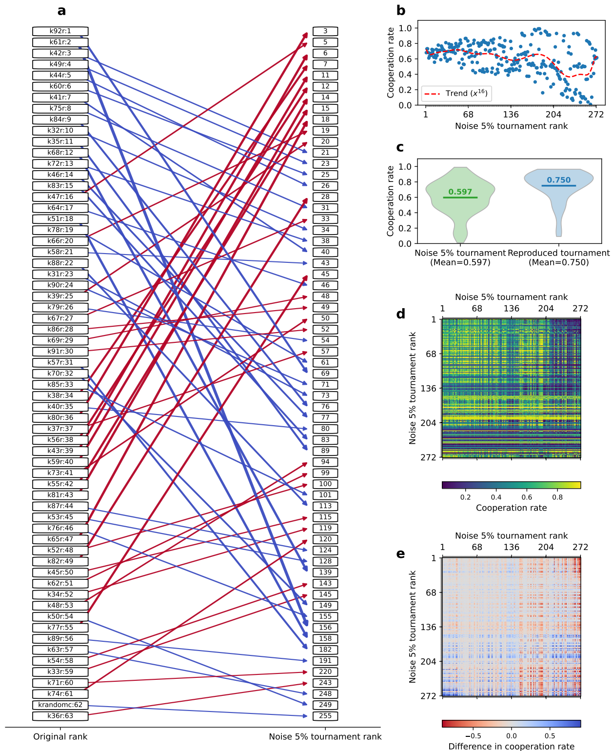
Figure 10: Reproduction of Axelrod's second tournament with the addition of the strategies from the Axelrod-Python and with noise 5%. Similar to Figure 6,
