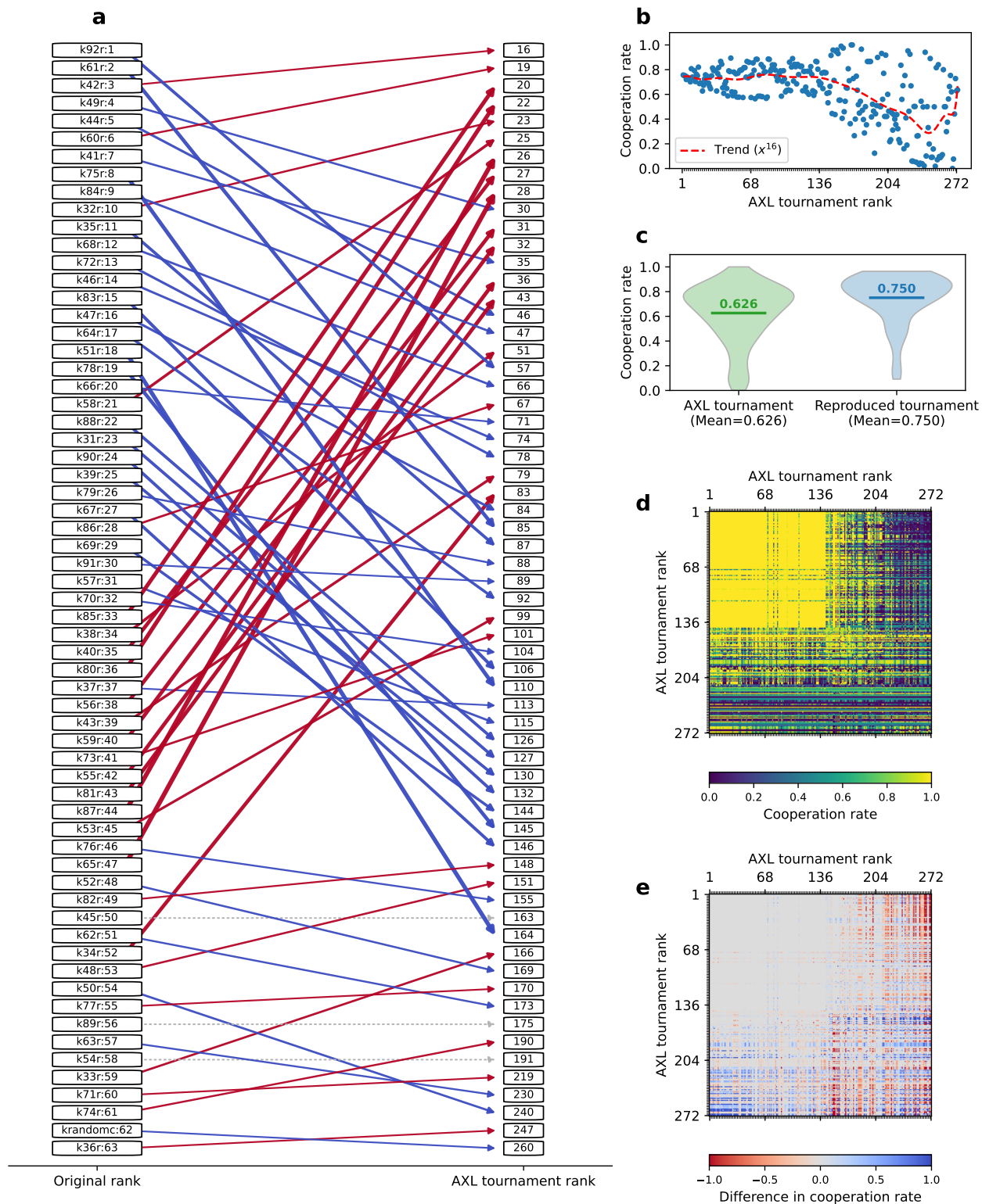
Figure 8: Reproduction of Axelrod's second tournament with the addition of the strategies from the Axelrod-Python. Similar to Figure 6,
