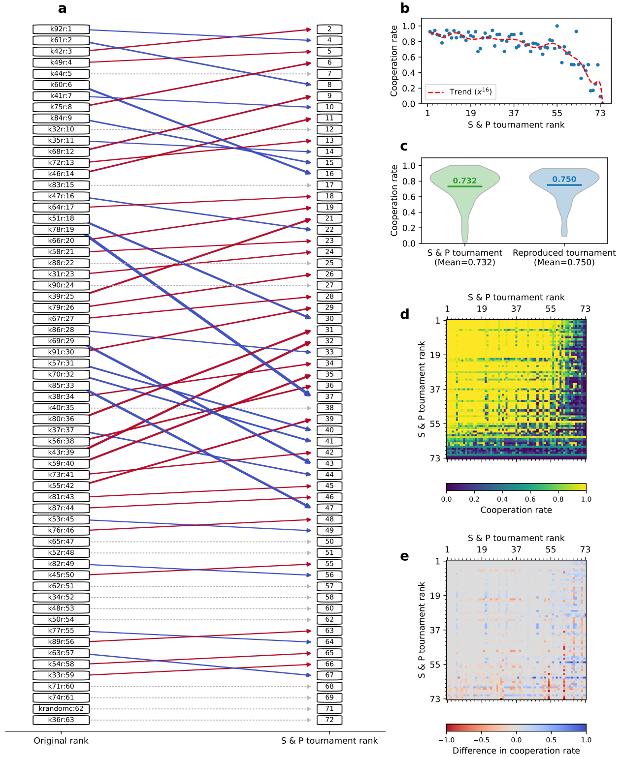
Figure 7: Reproduction of Axelrod's second tournament with the addition of the strategies from Stewart's and Plotkin's tournament [16]. Similar to Figure 6. Here we only show the new ranking of the original strategies. a , Comparison of the original rankings with those obtained in our replication with the addition of the strategies from [16]. b , Cooperation rates of strategies ordered by rank in the reproduced tournament with the additional strategies. c , Tournament ranks across all repetitions compared to the reproduced tournament without the additional strategies. We also plot the average cooperation rate. d , Pairwise cooperation rates between strategies. e , Differences in cooperation rates for each pair of strategies.
