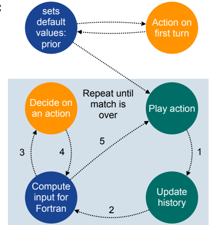
Fig. 1: Reviving Axelrod’s second tournament code. a , Fortran code for TFT ( k92r.f ). Each strategy takes as input the match state (J: opponent’s previous move; M: current turn number; K: player’s cumulative score; L: opponent’s cumulative score; R: random number in [0, 1] ; JA: player’s previous move) and returns 0 (cooperate) or 1 (defect). b , Overview of how the three codebases interact. Axelrod_fortran creates strategy instances for each player. Tournaments and matches are managed by Axelrod-Python , which, at each turn, calls the corresponding Axelrod_fortran instance; this, in turn, invokes the original Fortran code to produce a decision from the match history. c , Turn-by-turn execution. On the first turn, Axelrod_fortran initializes the parameters required by the Fortran implementation, queries it for a decision, and returns the move to Axelrod-Python , which plays it and updates the history. On each subsequent turn: (1) the previous outcome is recorded and the history updated; (2) Axelrod_fortran accesses the updated history; (3) formats it into the inputs expected by the Fortran code; (4) calls the Fortran function and receives a decision; and (5) Axelrod-Python plays the decision. The process repeats until the match ends.
