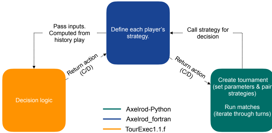
Fig. 1: Reviving Axelrod’s second tournament code. a , Fortran code for TFT ( k92r.f ). Each strategy takes as input the match state (J: opponent’s previous move; M: current turn number; K: player’s cumulative score; L: opponent’s cumulative score; R: random number in [0, 1] ; JA: player’s previous move) and returns 0 (cooperate) or 1 (defect). b , Overview of how the three codebases interact. Axelrod_fortran creates strategy instances for each player. Tournaments and matches are managed by Axelrod-Python , which, at each turn, calls the corresponding Axelrod_fortran instance; this, in turn, invokes the original Fortran code to produce a decision from the match history. c , Turn-by-turn execution. On the first turn, Axelrod_fortran initializes the parameters required by the Fortran implementation, queries it for a decision, and returns the move to Axelrod-Python , which plays it and updates the history. On each subsequent turn: (1) the previous outcome is recorded and the history updated; (2) Axelrod_fortran accesses the updated history; (3) formats it into the inputs expected by the Fortran code; (4) calls the Fortran function and receives a decision; and (5) Axelrod-Python plays the decision. The process repeats until the match ends.
