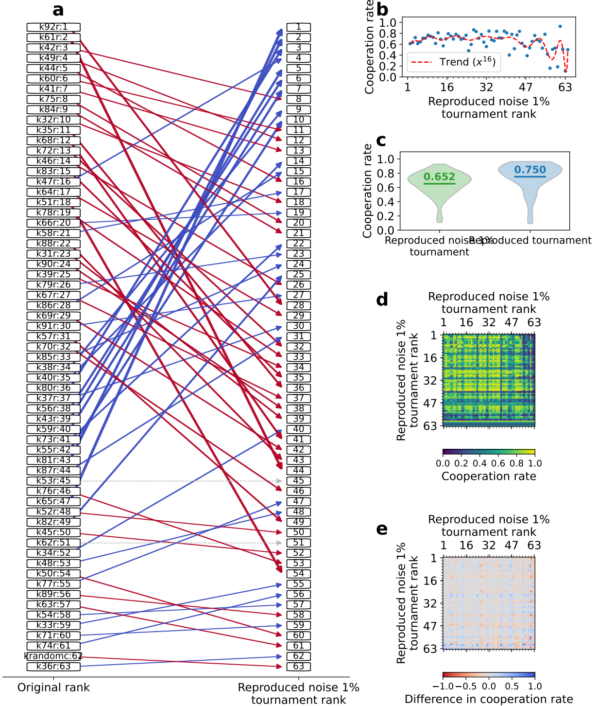
Fig. 5: Axelrod's second tournament with 1% noise. a , Comparison of the original rankings and the rankings of the second tournament with noise. In the left column, strategies are ordered by their original ranks, and arrows indicate their ranks in the noisy tournament (right column). The arrow widths are proportional to the change in rank. Blue arrows indicate a positive change in rank, red arrows indicate a negative change in rank, and grey arrows indicate no change in rank. b , Cooperation rates of strategies ordered by rank in this tournament. c , Tournament cooperation rates across all repetitions for this tournament (green) and the reproduced tournament without noise (blue). We also plot the average cooperation rate (green or blue line) and report its value. d , Pairwise cooperation rates between strategies. For each pair we calculate the cooperation rate of the row strategy towards the column strategy and vice versa. The strategies are ordered by the ranks in this tournament. For a full list of strategies see Supplementary Table 2, Supplementary Table 4, and Supplementary Information (S8) . e , Differences in cooperation rates for each pair of strategies, again ordered by their rank in the reproduced tournament with noise.
