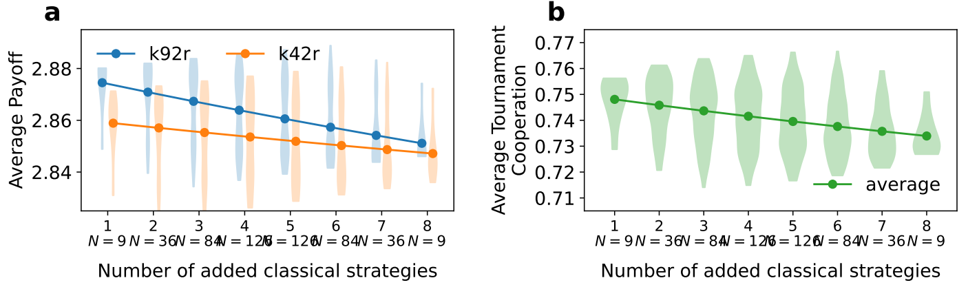
Fig. 4: Effect of additional classical strategies on average payoffs and tournament cooperation. a , Distributions of the average tournament payoffs achieved by TFT (k92r) and k42r as a function of the number of added classical strategies. Violins show the distribution of outcomes across all possible combinations of additional invitees, while lines indicate the mean payoff for each subset size. b , Distribution of the average cooperation levels across tournaments for each subset size. Intermediate subset sizes produce the widest cooperation distributions, indicating greater diversity in the resulting tournament interactions. These are also the conditions under which TFT performs least effectively relative to k42r. All tournaments use the original tournament setting of five fixed match lengths and are repeated 250 times.
