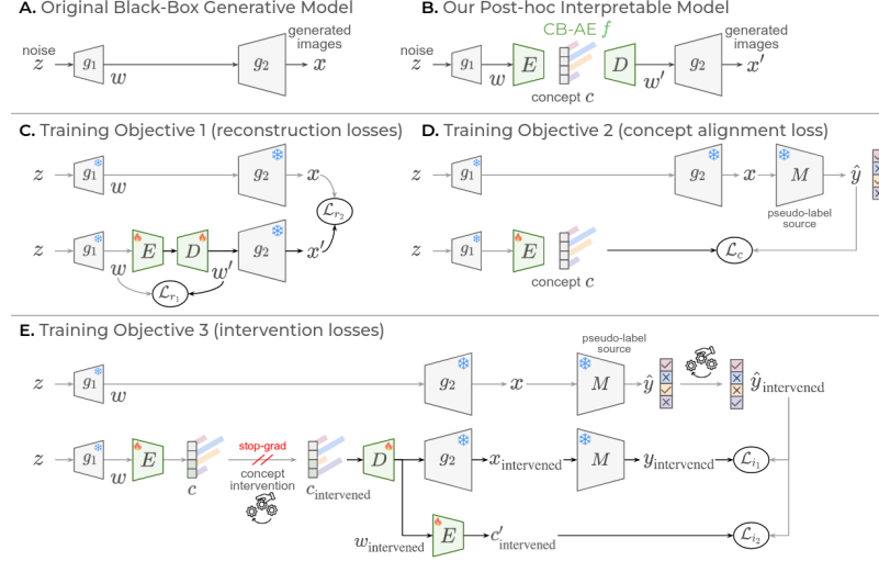
Figure 9: Architecture of the Post-hoc Concept Bottleneck Generative Model where the different loss functions are illustrated.
