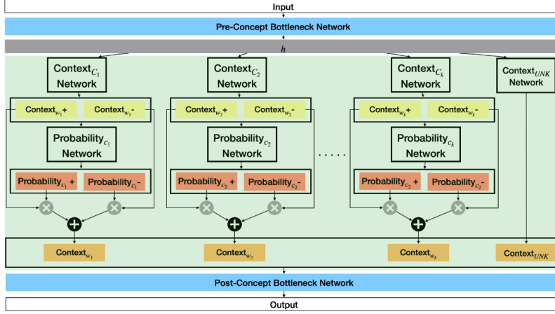
Figure 8: Architecture of the concept layer in the Concept Bottleneck Generative Model (CBGM) for a generic generative model.
