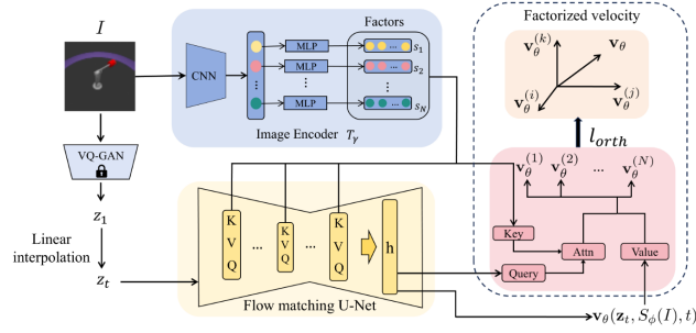
(b) FM Disentanglement Framework
