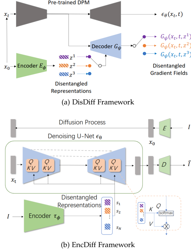
Figure 5: Illustrations of the frameworks for the (a) DisDiff model [42] and the (b) EncDiff model. [41]
