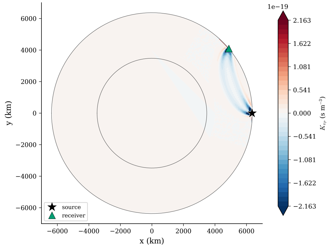
1-D PREM: v_P traveltime sensitivity kernel (P400P)
