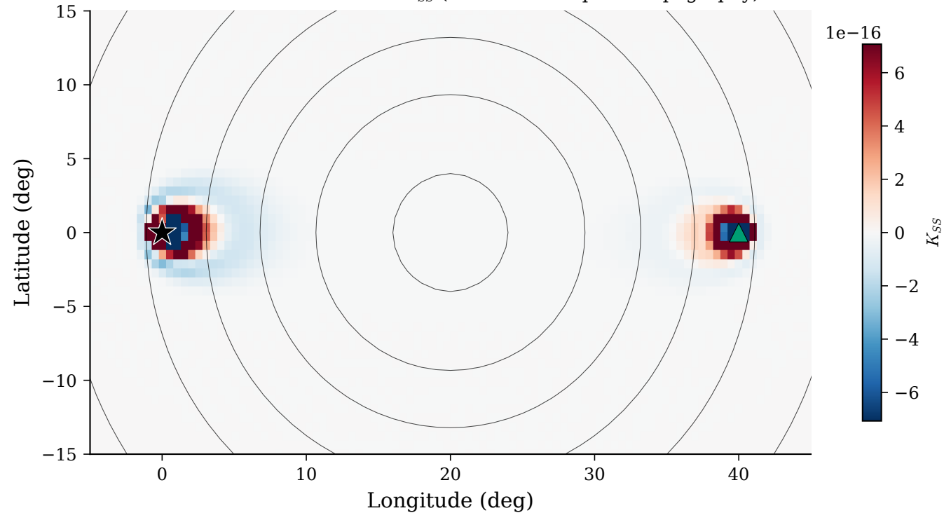
3-D: Moho interface kernel K_{SS} (contours = imposed topography)
