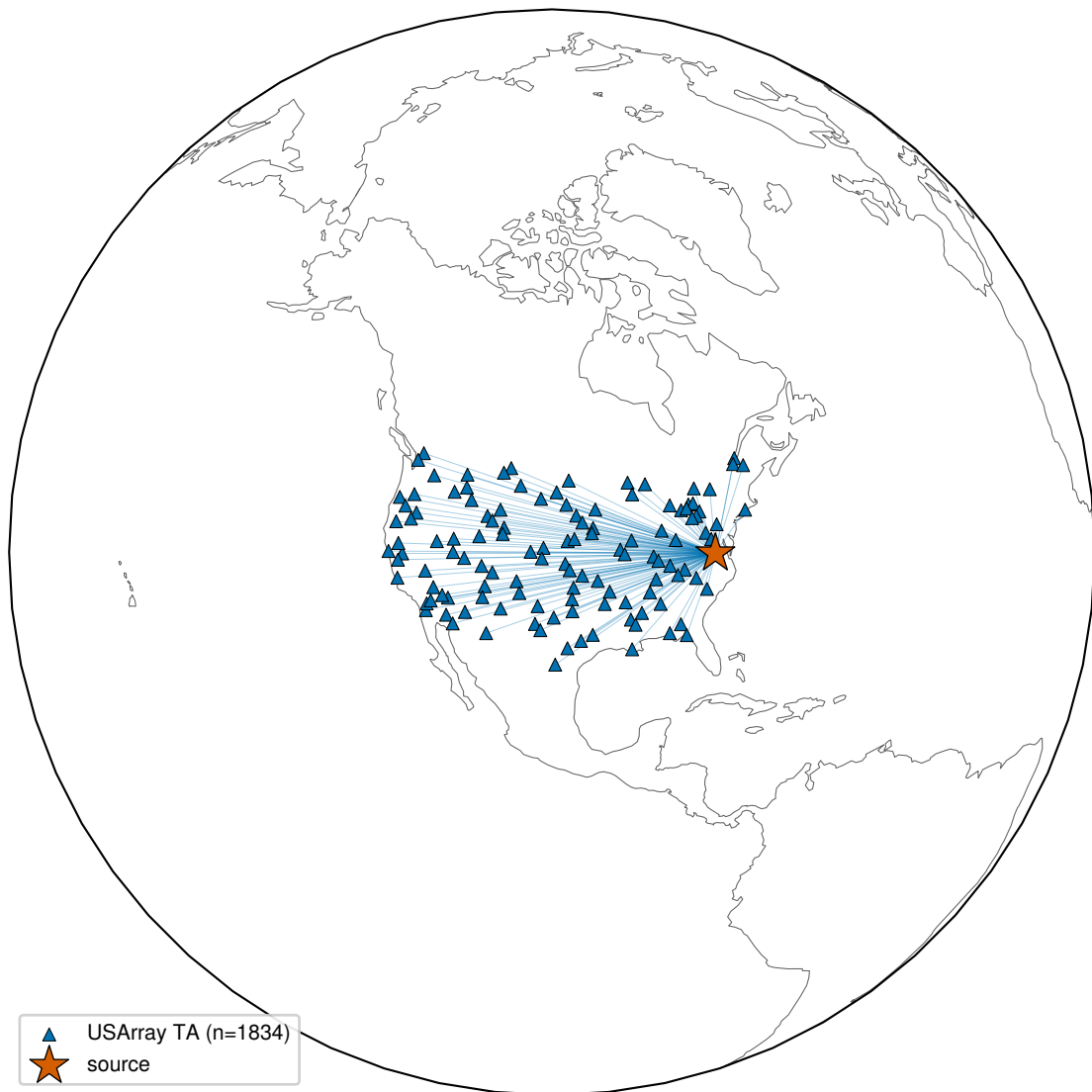
Virginia 2011 + USArray TA — source-receiver geometry
