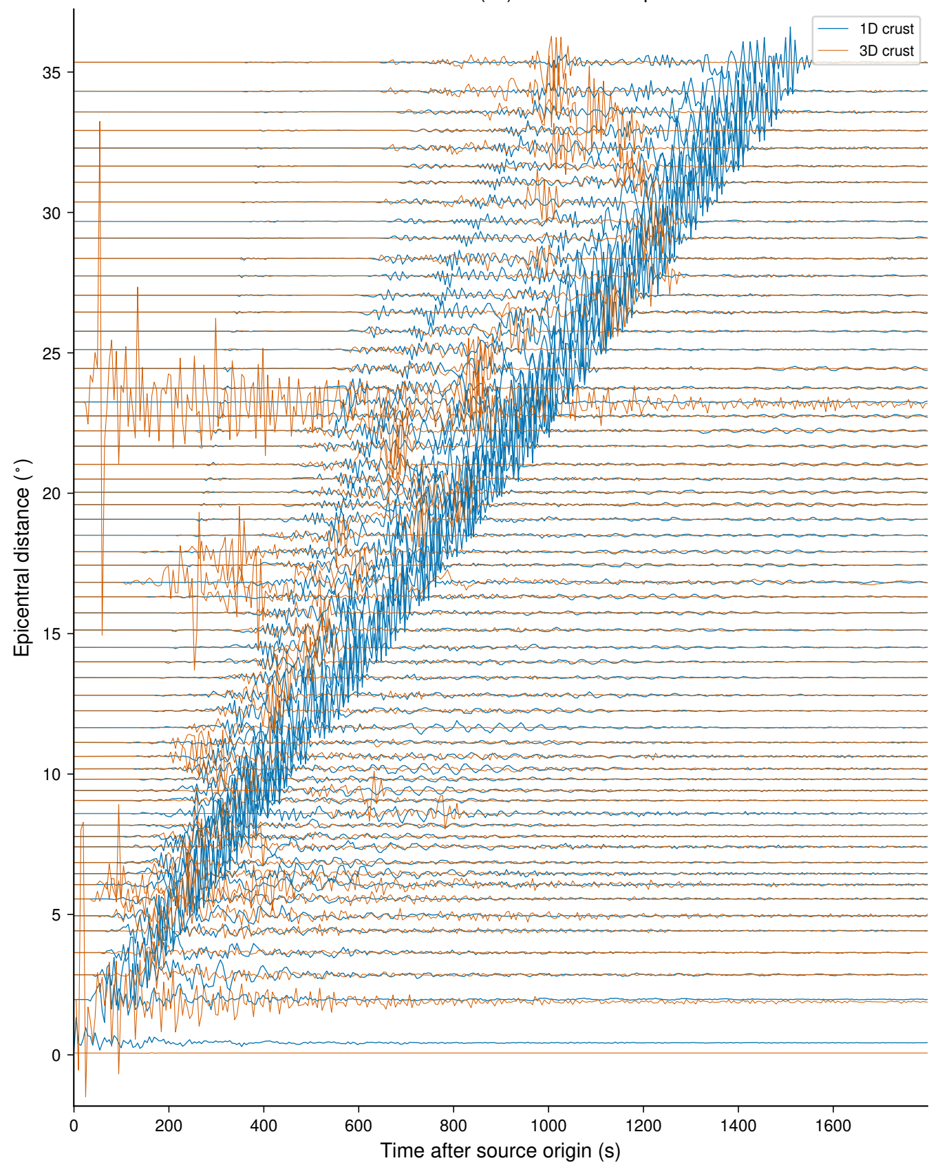
1D vs 3D crustal model (5s) — Vertical displacement
