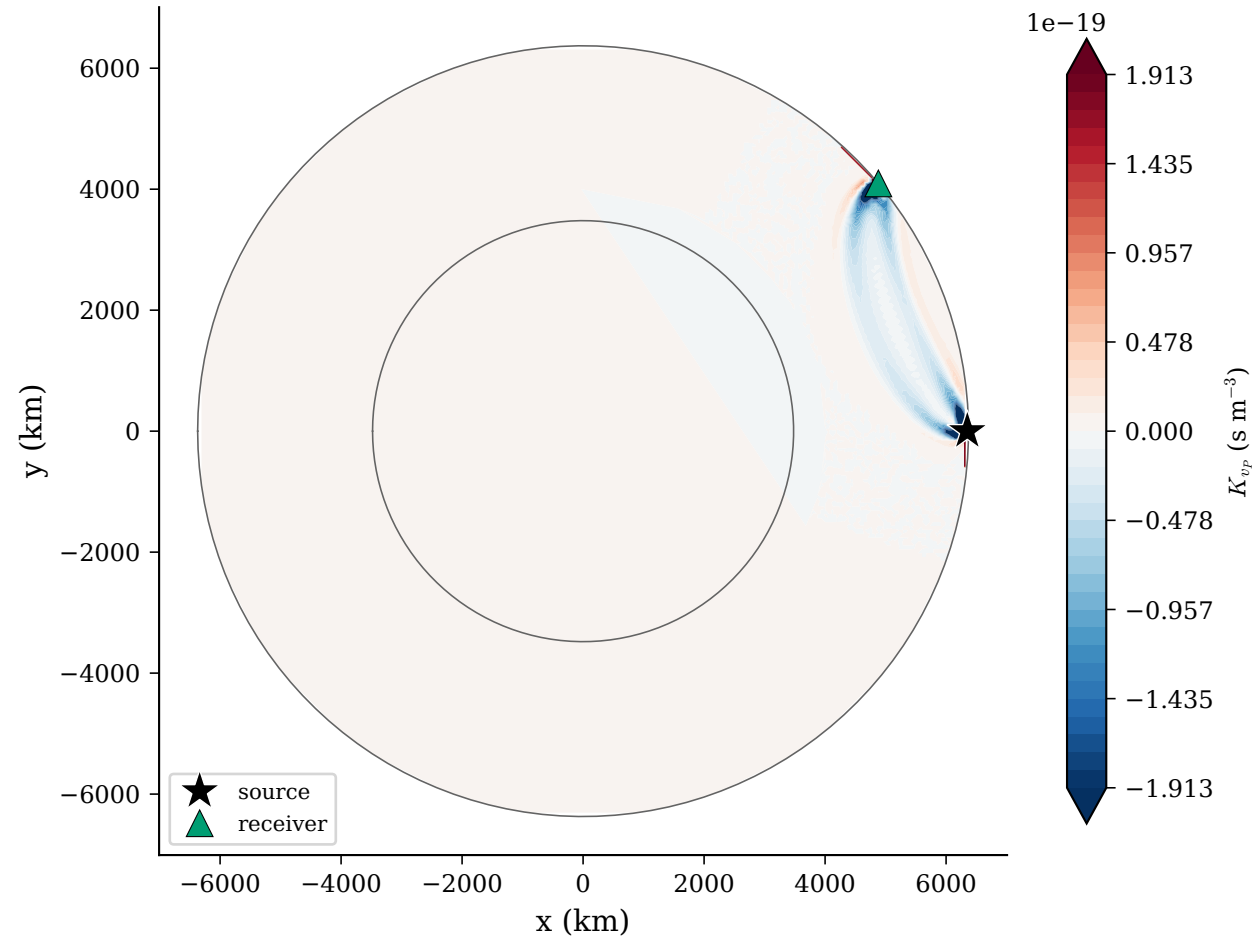
3-D (S362ANI + Moho): v_P traveltime kernel (P400P)
