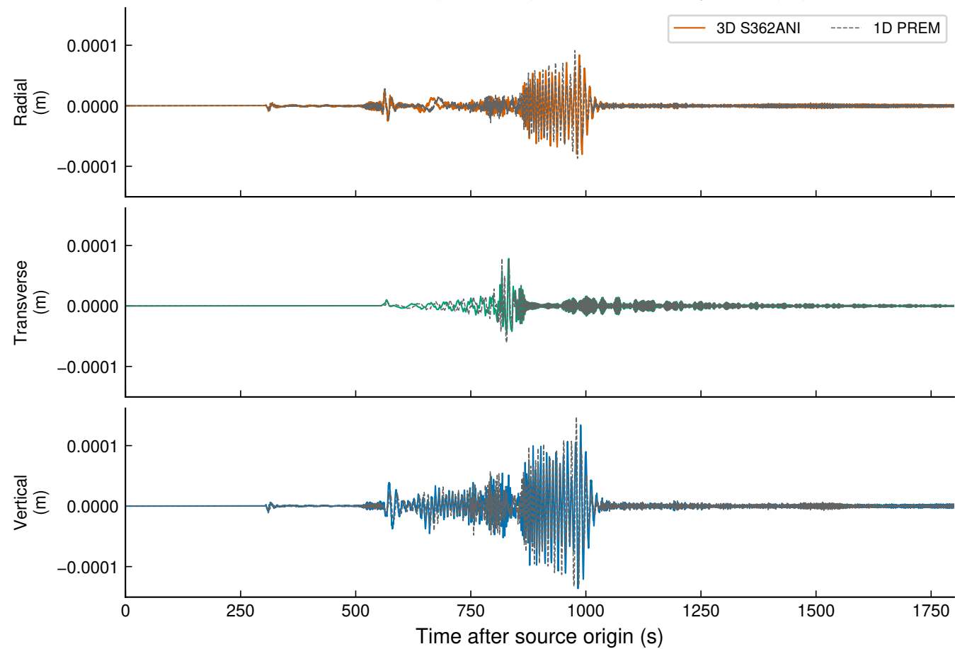
Station IU.ANMO ( \Delta = 23.1^\circ ) — 1D vs 3D comparison (5s)
