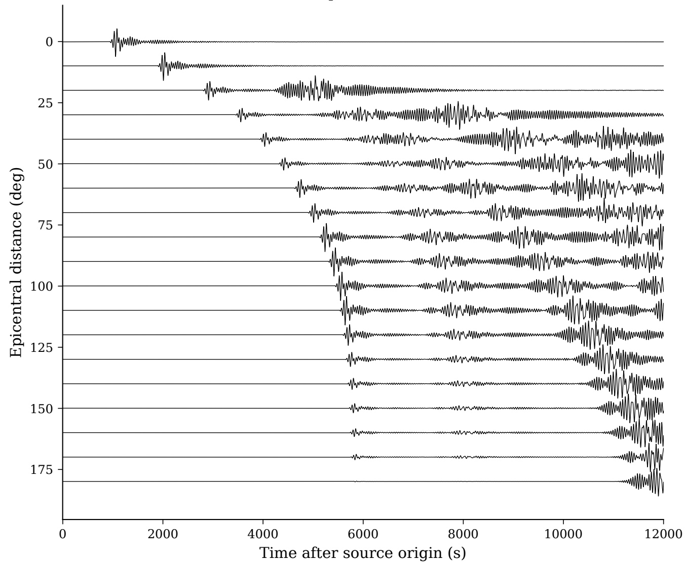
Sun: vertical-displacement record section
