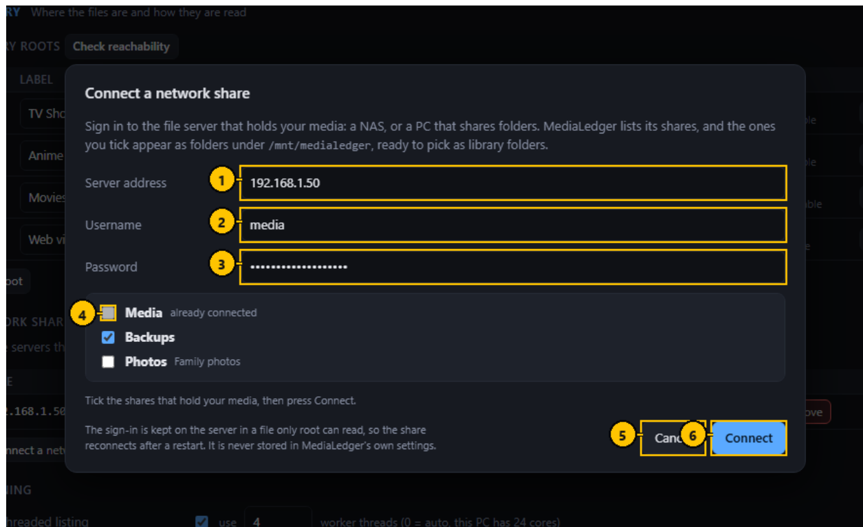
Figure 4. The connect dialog after Find shares: one share already connected, one ticked.
