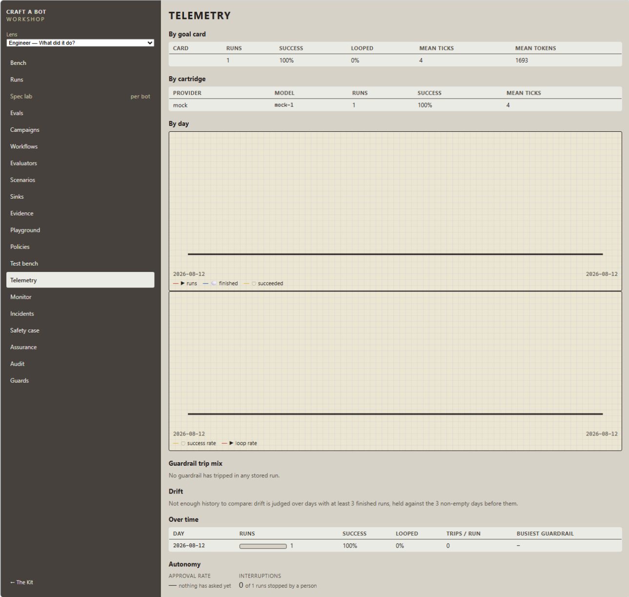
Figure 13 – Telemetry, with drift
