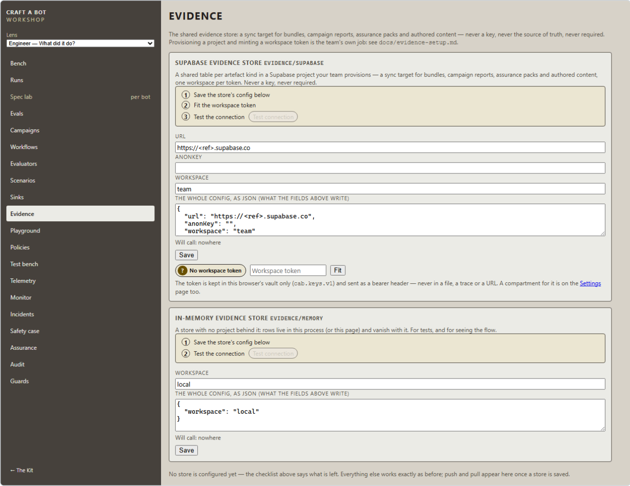
Figure 15 — The Evidence screen
