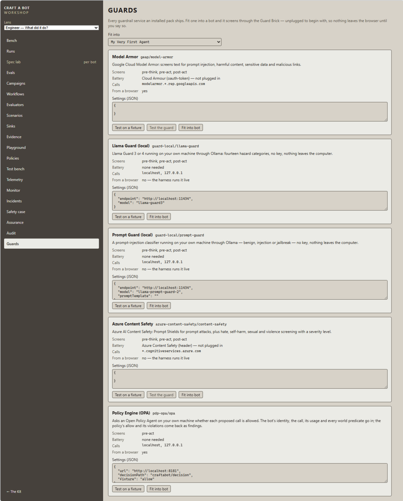
Figure 12 – The Guard Rack
