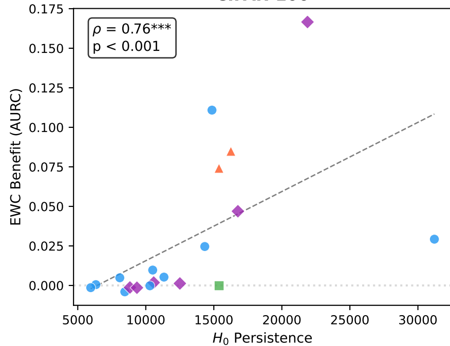
CIFAR-100
