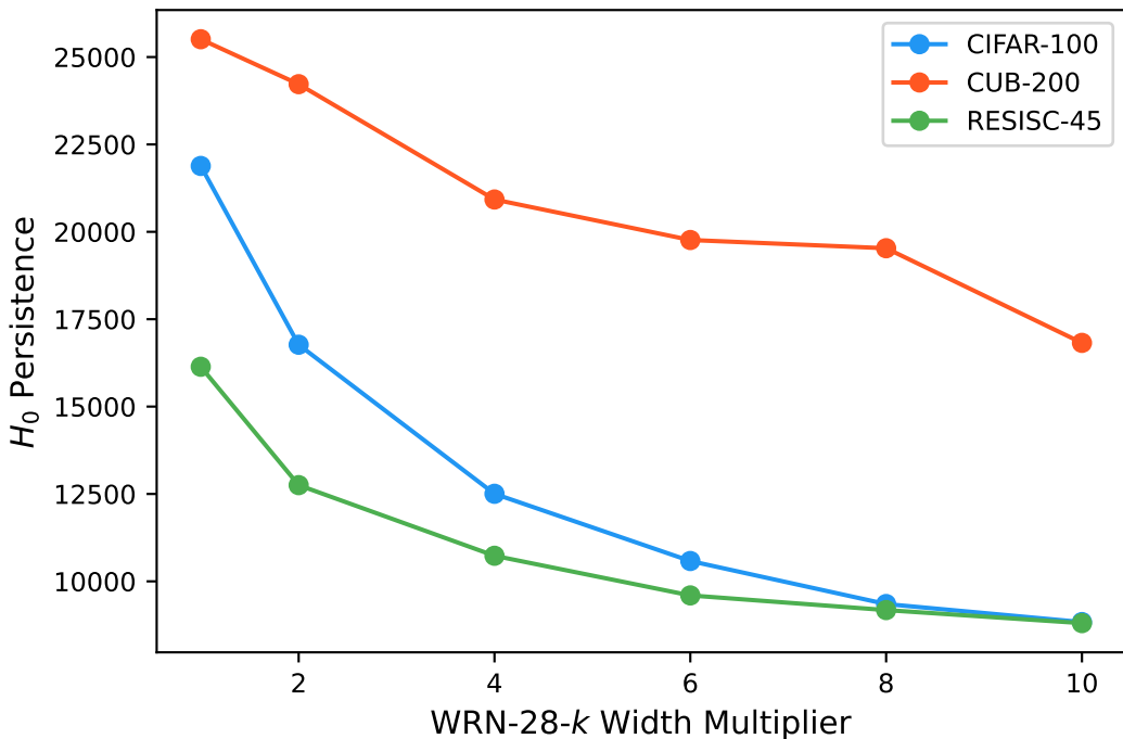
H_0 Decreases Monotonically with Width ( \rho = -1.0 )
