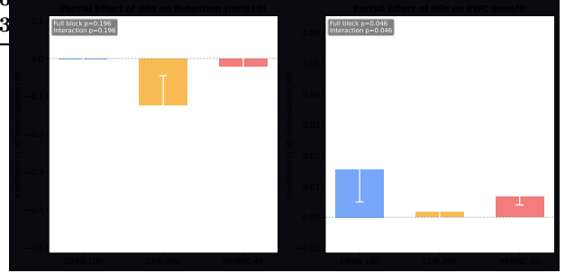
Figure 1: Per-dataset partial effects of within-dataset \tilde{H}_0 with 95% clustered bootstrap CIs. Left: effect on retention (ret@10); the CUB-200 effect excludes zero. Right: effect on EWC benefit; CIFAR-100 and RESISC-45 effects exclude zero while CUB-200 does not, demonstrating dataset moderation (block permutation p = 0.046 ).
