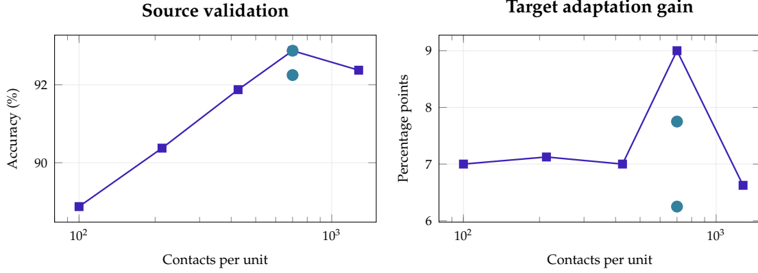
Figure 17: SHD adaptation as the number of synaptic contacts changes. The development result on one source is non-monotonic; two independently trained sources confirm the selected 700-contact setting.
