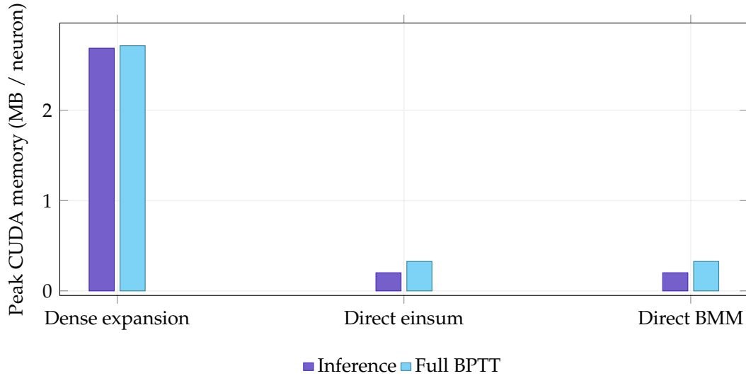
Figure 19: Peak CUDA memory per neuron for inference and full BPTT across dense branch expansion, direct einsum, and direct BMM contact-input implementations at 24 contacts and 256 timesteps.
