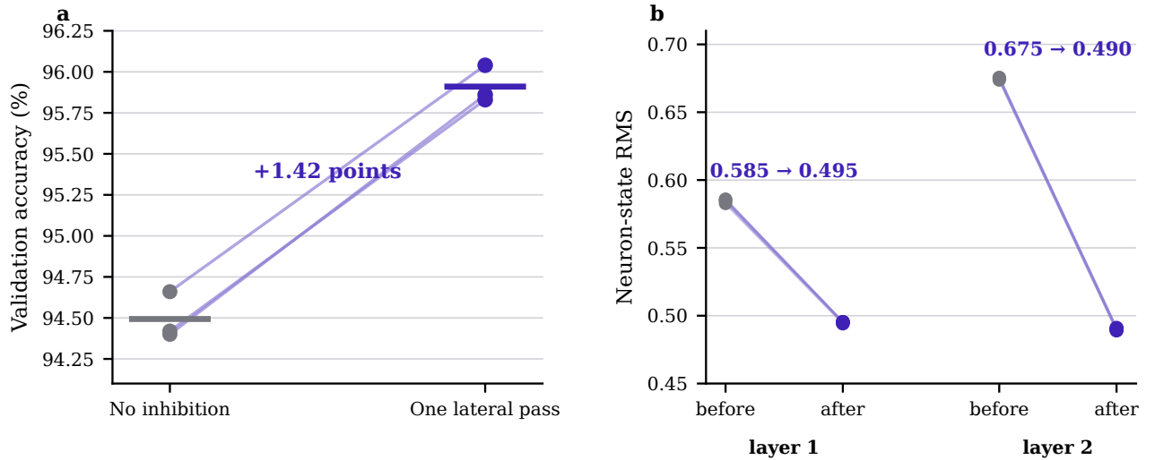
Figure 2: Effect of residual-state inhibition. a , One lateral pass improves each matched validation run over the otherwise identical no-inhibition rule; horizontal bars show means. b , The same pass reduces the population RMS of the neuron state in both layers of every final run.
