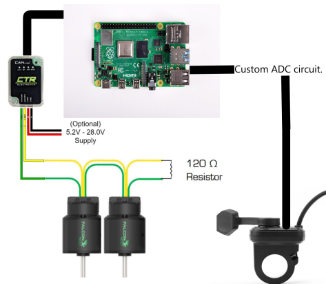
Figure 10: Electric Drivetrain Architecture.
